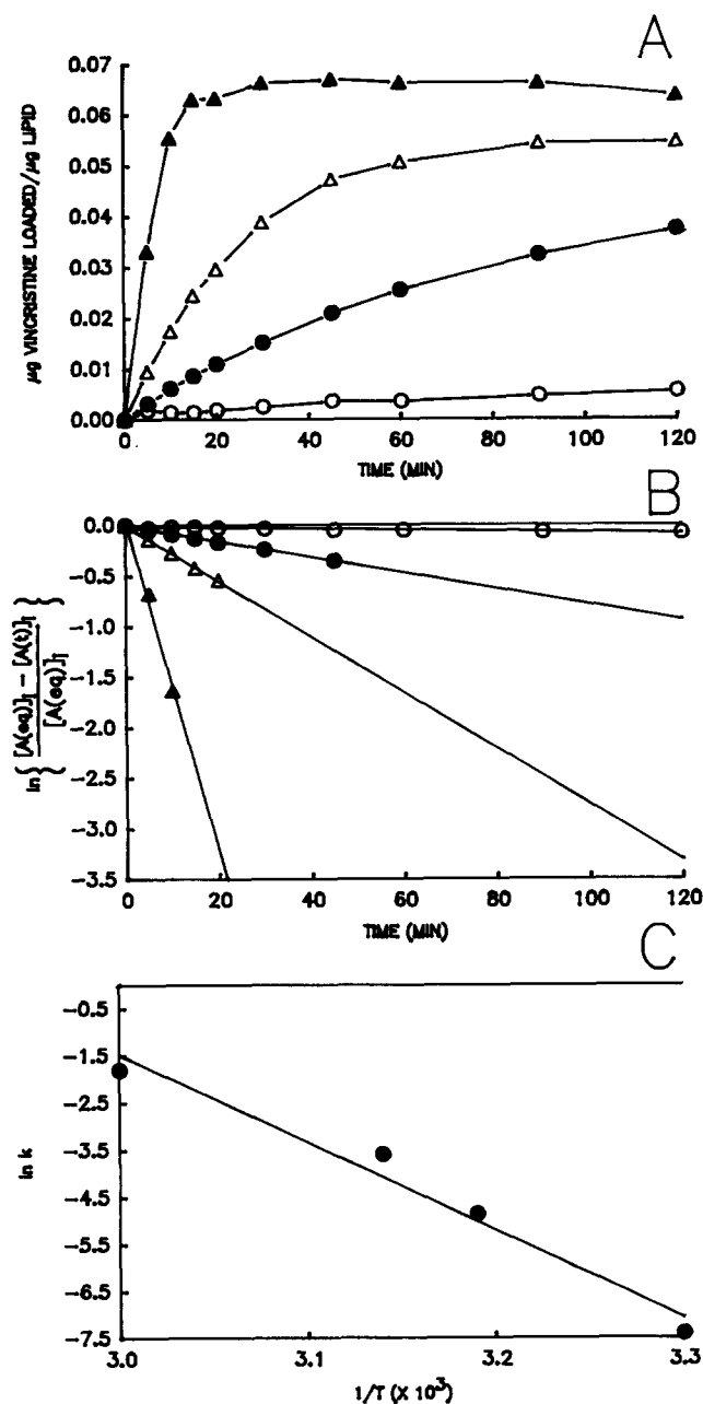
Fig. 4. (A) Time-course of vincristine uptake into 100-nm DSPC/Chol vesicles exhibiting a \Delta pH ( pH_i = 3.0 ; pH_o = 5.0 ). Uptake was conducted at 30 (○), 40 (●), 45 (△), and 60°C (▲). (B) Plot of \ln\{([A(eq)]_i - [A(t)]_i)/[A(eq)]_i\} vs. t , where [A(t)]_i and [A(eq)]_i are the same as for Fig. 2. (C) Arrhenius plot of the rate constants ( k ) for vincristine uptake. The activation energy calculated from the slope of this plot is 37 kcal/mol.
